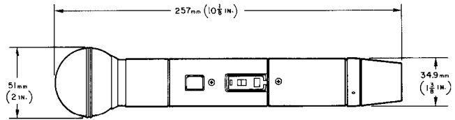
OVERALL DIMENSIONS FIGURE 7
