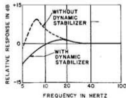
Typical Tone Arm-Cartridge Characteristics
