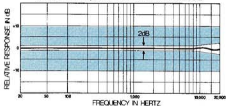
TYPICAL FREQUENCY RESPONSE ENVELOPE
