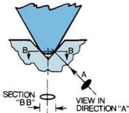
HYPERELLIPTICAL STYLUS OF THE V15 TYPE IV
