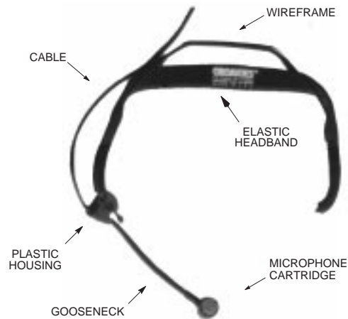
MICROPHONE PARTS
