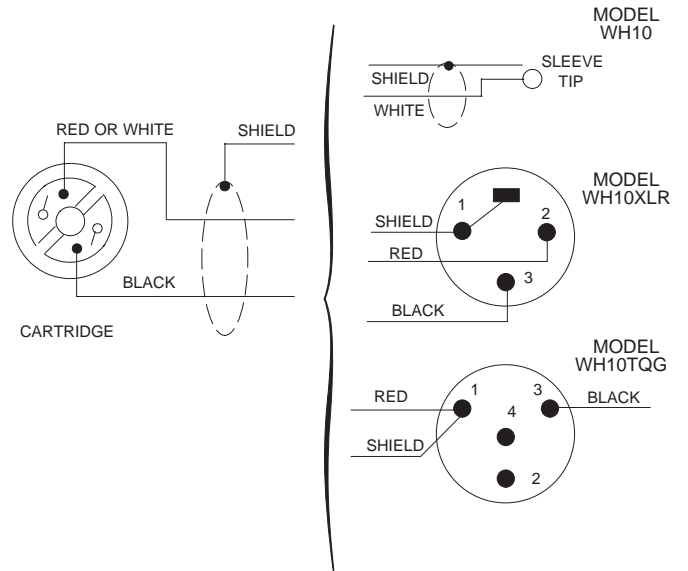
WIRING DIAGRAMS FIGURE 9
